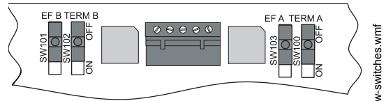
Figure 7 NCM-W Switches
